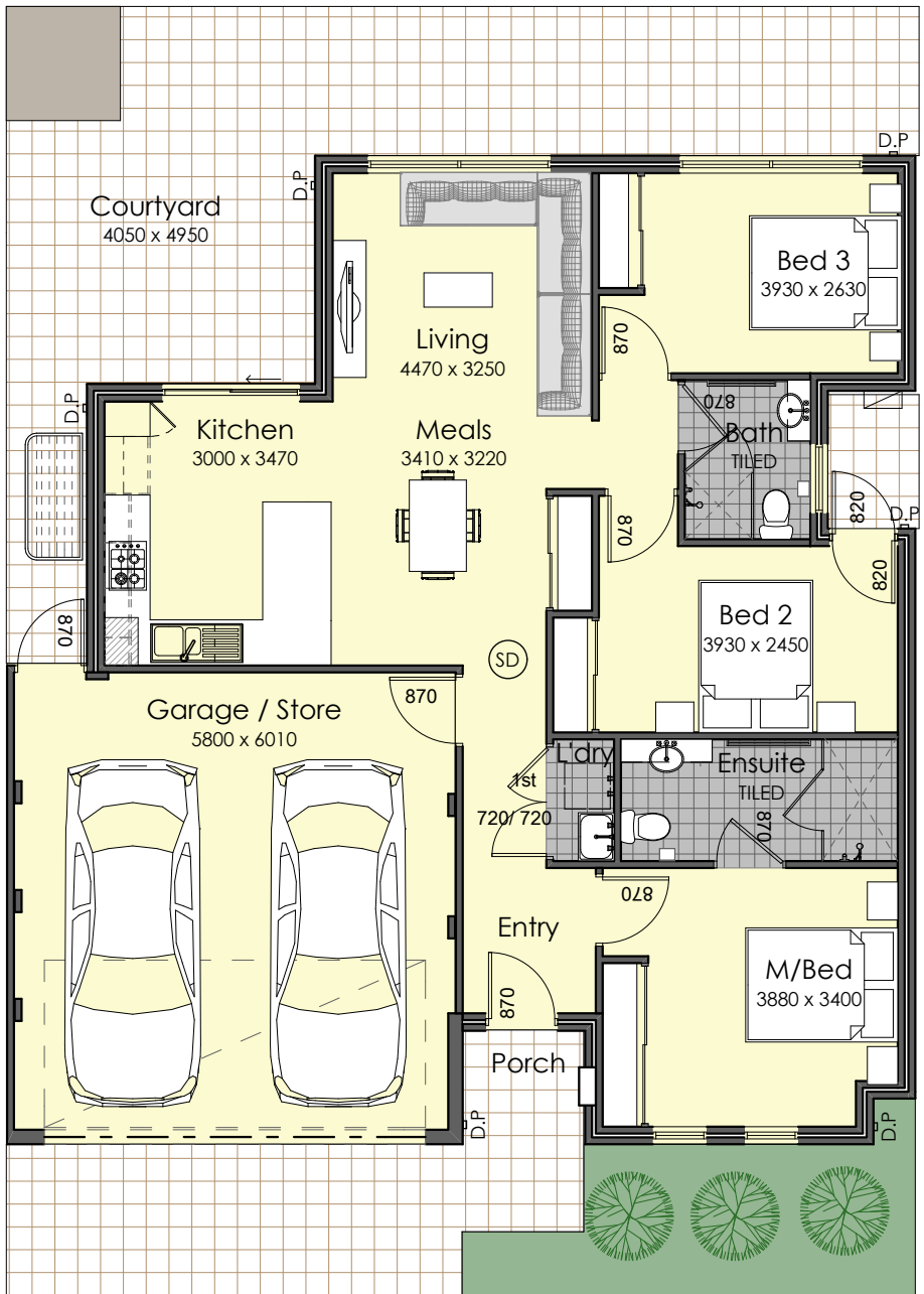
FLOOR PLAN 'TYPE E'
